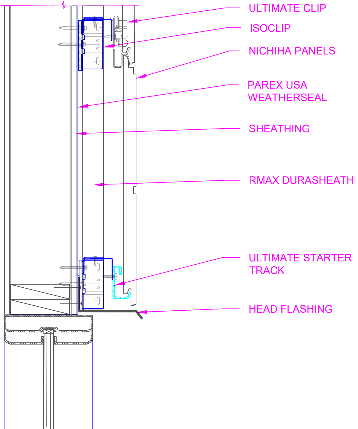
NICHIHA WINDOW HEAD WITH CI - FLUSH
